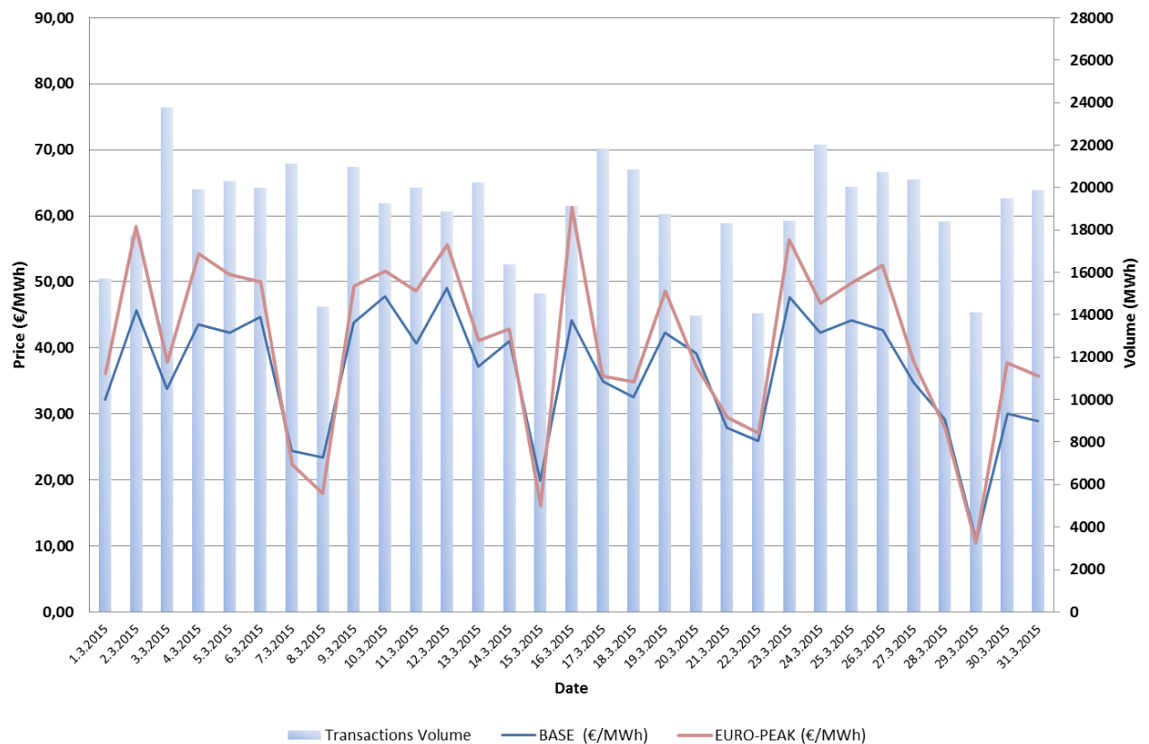
Slovenian Day-ahead Market Auction Prices and Volumes Delivery Day: 01.03.2015 – 31.03.2015
